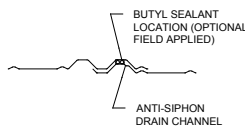
Correct AluTwin Sidelap
