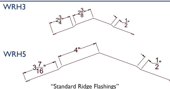
“Standard Ridge Flashings”
